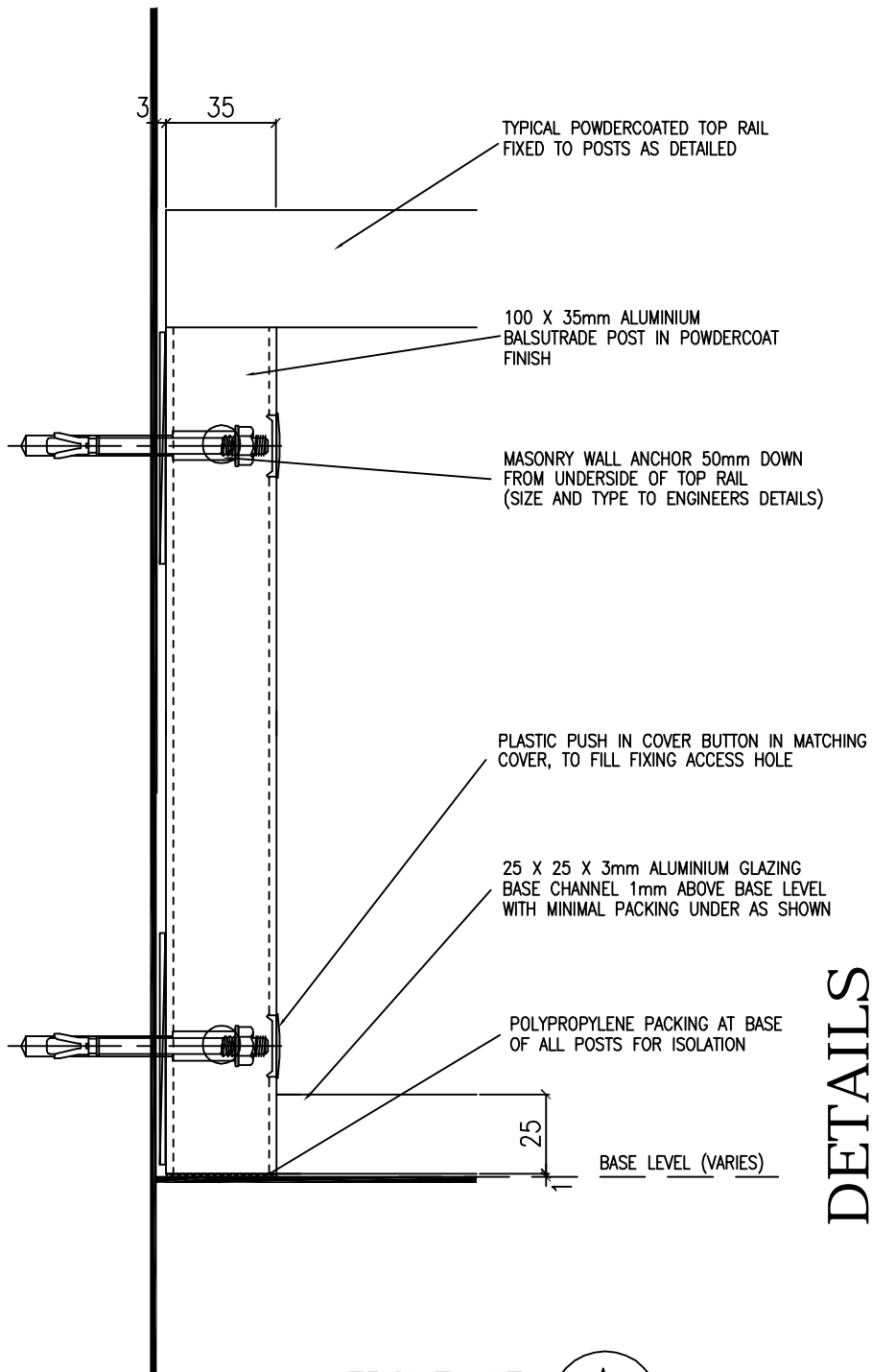
FRONT VIEW (A) MAY BE MIRRORED TO SUIT
